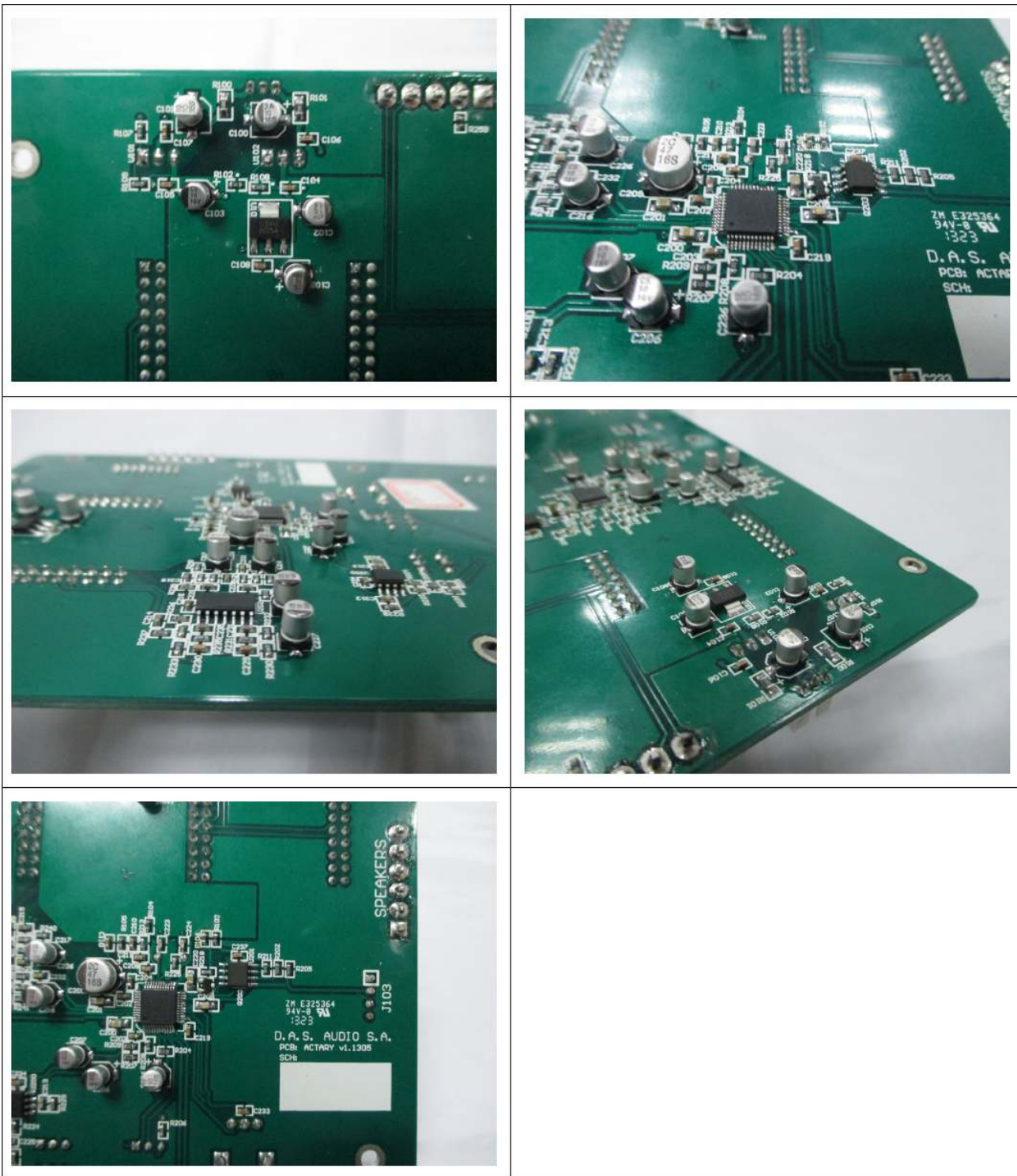
PCB for Controller
